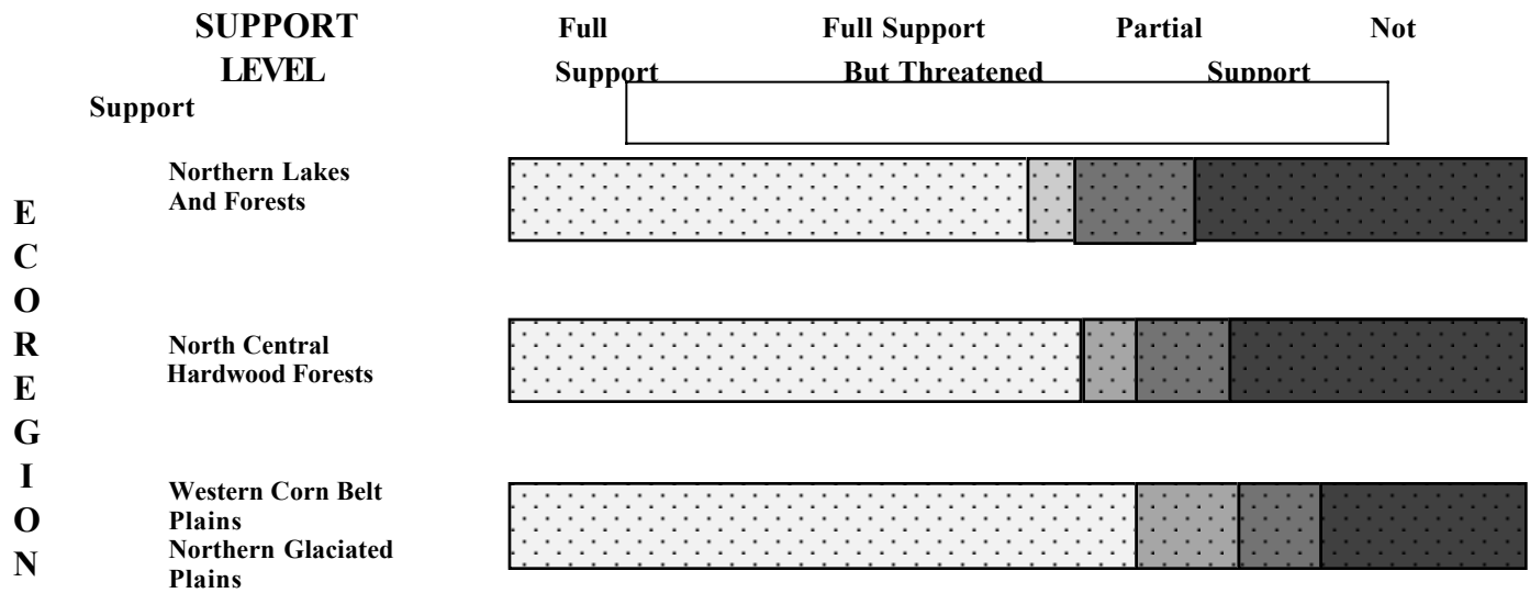
Figure 2. MPCA's Swimmable Use Support Classification Relative to Carlson's Trophic State Index by ecoregion.
