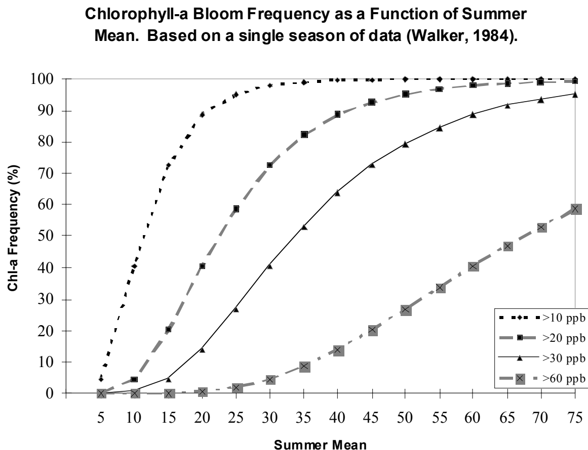
Figure 4. Chlorophyll-a Interval Frequency as a Function of Summer-Mean Chlorophyll-a.
